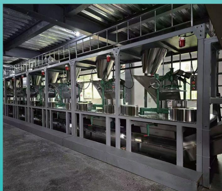
▲ AUTO TEA ROLLING GROUP
