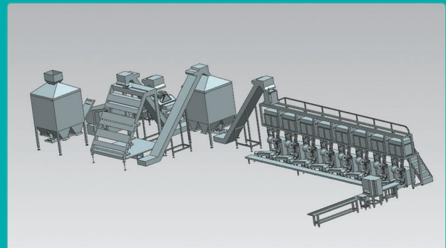
▲ TEA BLENDING & PACKAGING LINE
